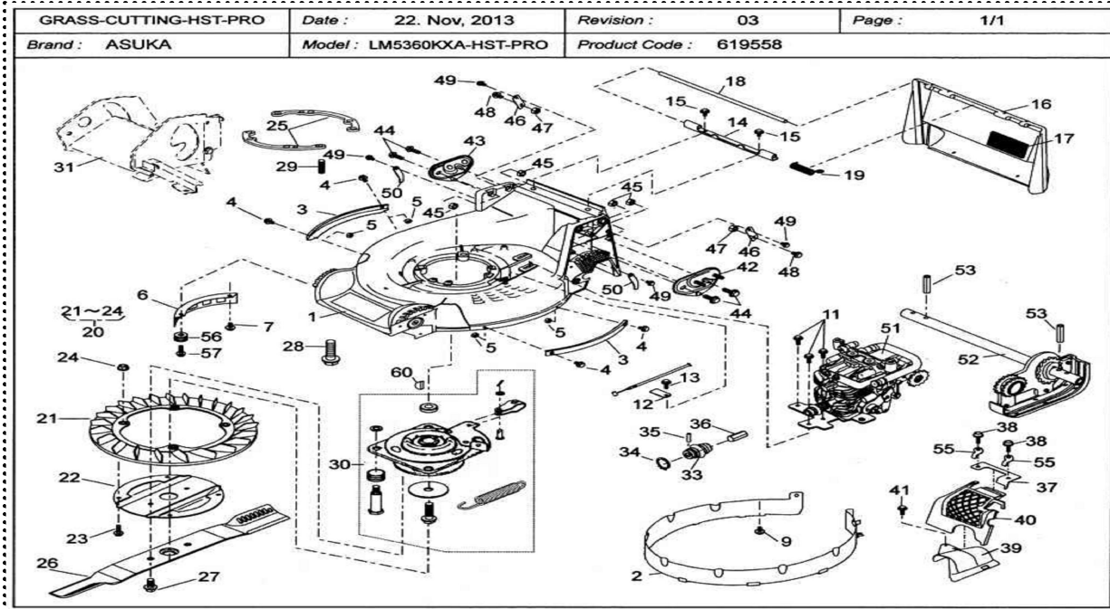
(A) LM5360KXA-HST-PRO
